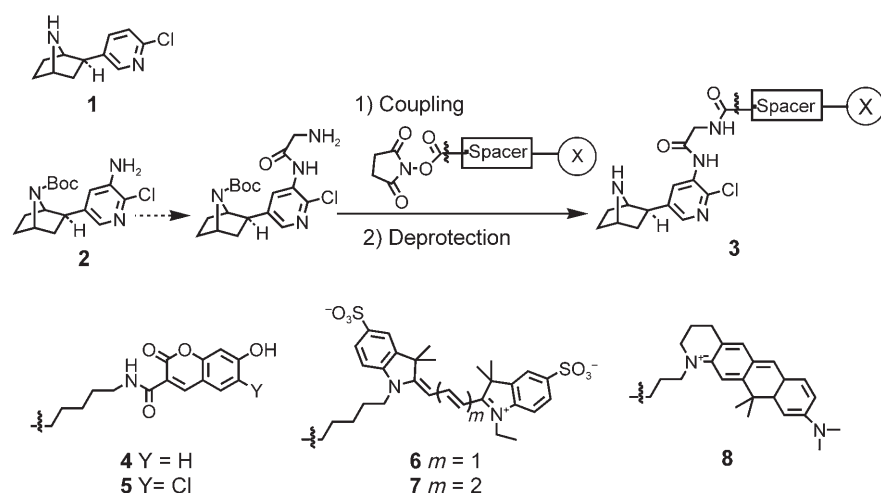
Scheme 1. Fluorophore conjugation to EPB (1). 7-Boc-3'-aminoepibatidine (2; Boc: tert -butoxycarbonyl) was first modified with an aminoacyl linker and then reacted with an N -hydroxysuccinimide-activated fluorophore X to yield after deprotection a fluorescent EPB (3); X: coumarin (EPB-Cou, 4), 6-chlorocoumarin (EPB-Cl-Cou, 5), Cy3 (EPB-Cy3, 6), Cy5 (EPB-Cy5, 7), Atto610 (EPB-Atto610, 8). For details, see the Supporting Information.
